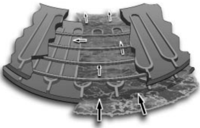
Disc filtration flow
