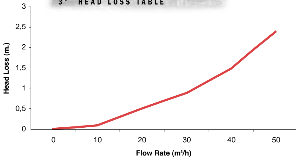
3" HEAD LOSS TABLE
