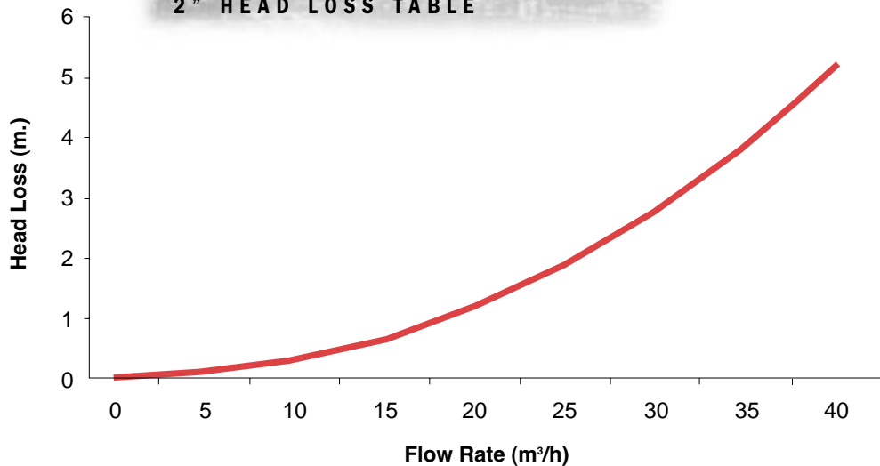
2" HEAD LOSS TABLE
